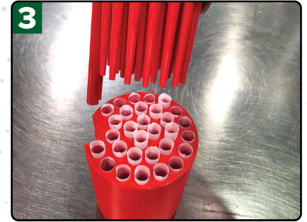
3 Seat in the cones with the pushing tool
